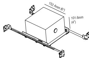
IC064R01060 Recessed Box for Insulated Ceiling with 60mm Hole
