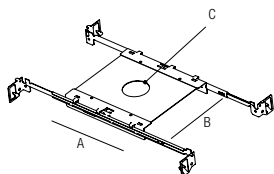
R01060 Mounting Plate with 60mm Hole
