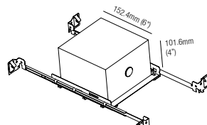
IC064R01040 Recessed Box for Insulated Ceiling with 40mm Hole
