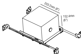
IC086Q02080 Recessed Box for Insulated Ceiling with 80mm Hole
