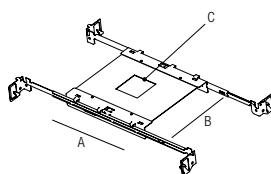
Q02080 Mounting Plate with 80mm Hole
